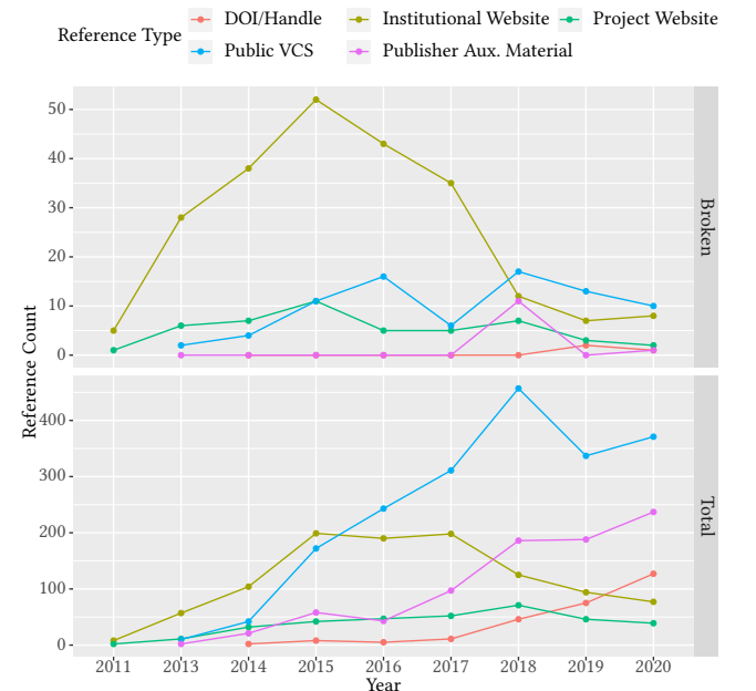
Figure 4: Total and broken artifact links according to HTTP response for different platforms
